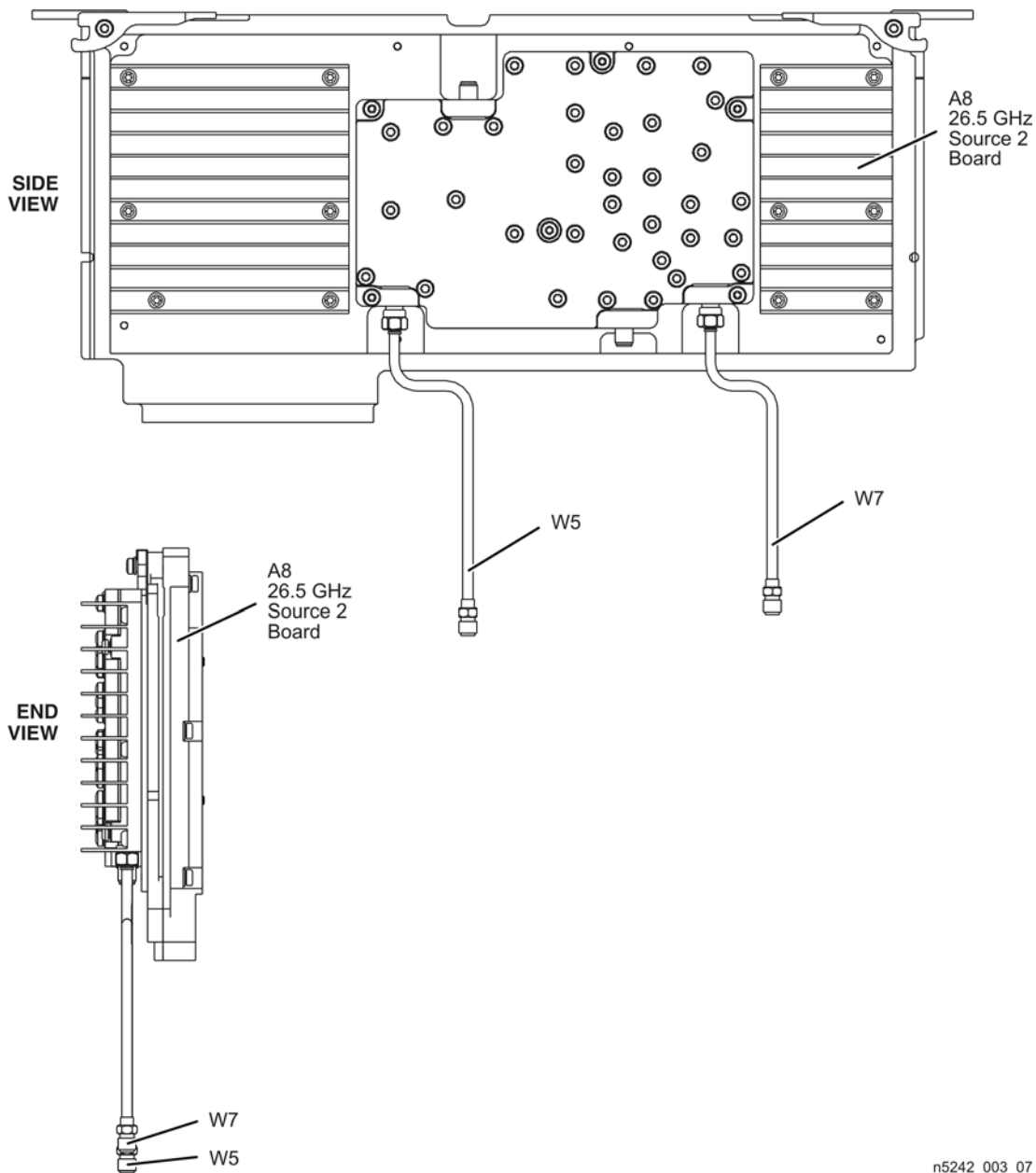
Figure 8 Cable Connections to the Second Source Boards, Part 1b
