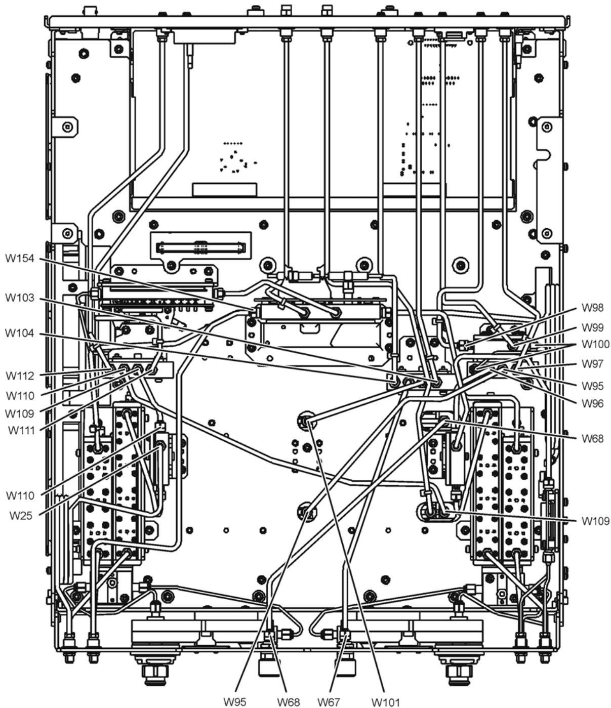
Figure 14 New Test Set Cable Installation
