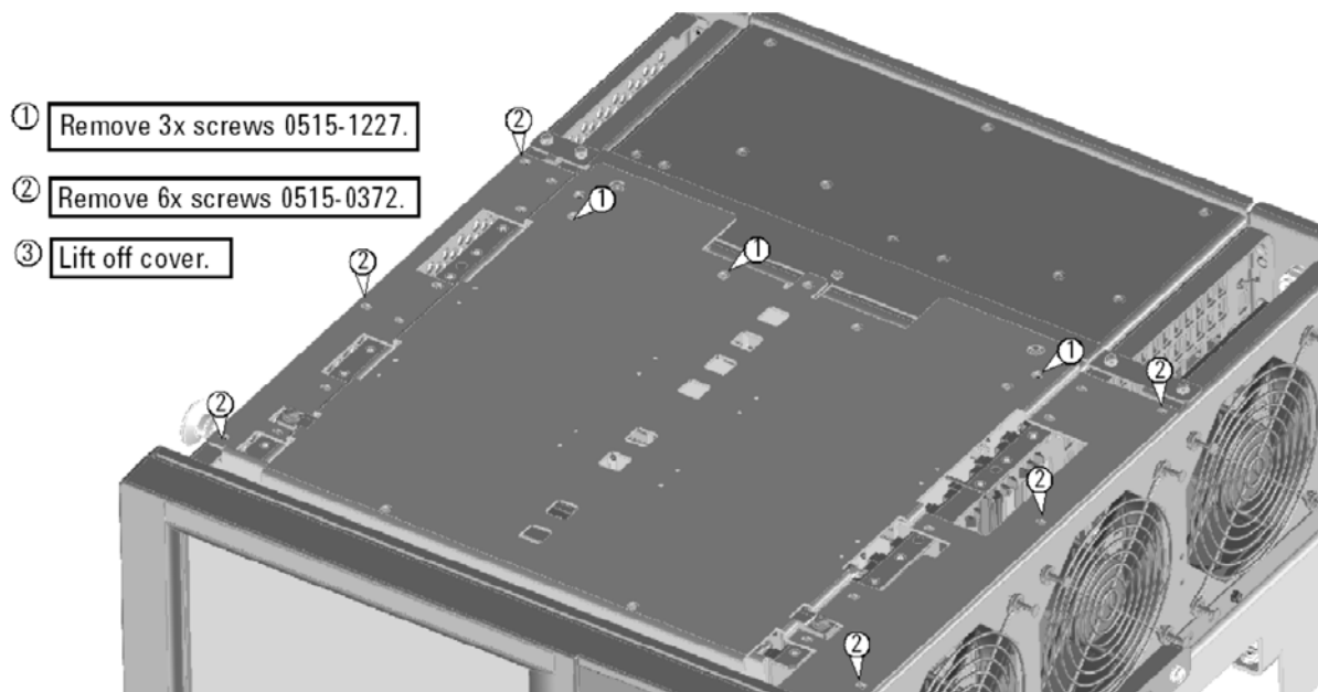
Figure 2 Inner Cover Removal
