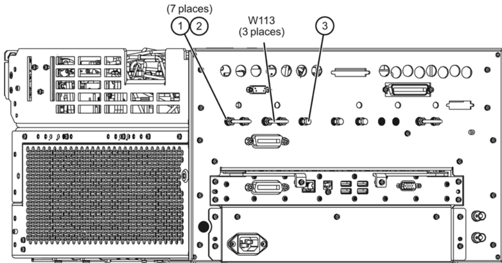
Figure 13 Bulkhead Connectors and Jumpers on Rear Panel
