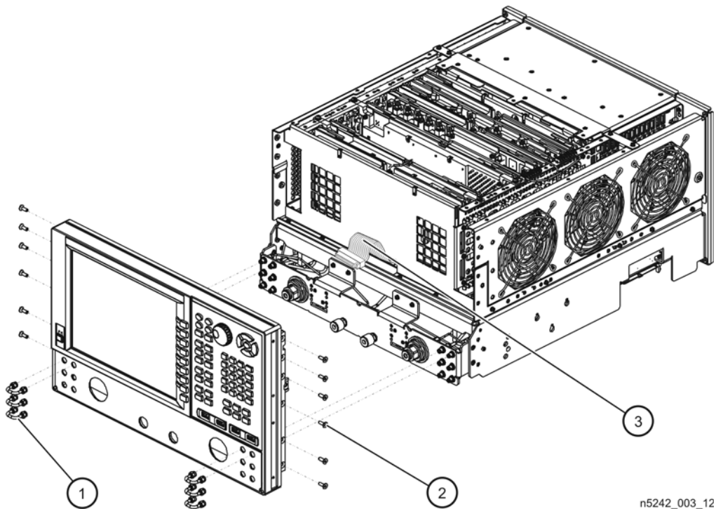
Figure 18 Front Panel Assembly Reinstallation
