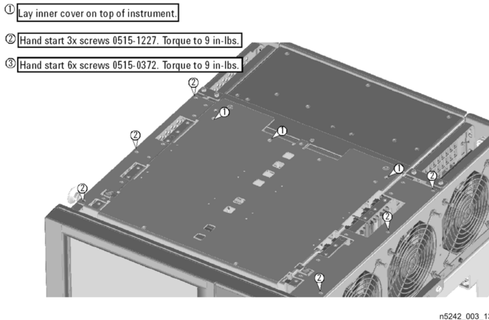
Figure 19 Inner Cover Reinstallation
