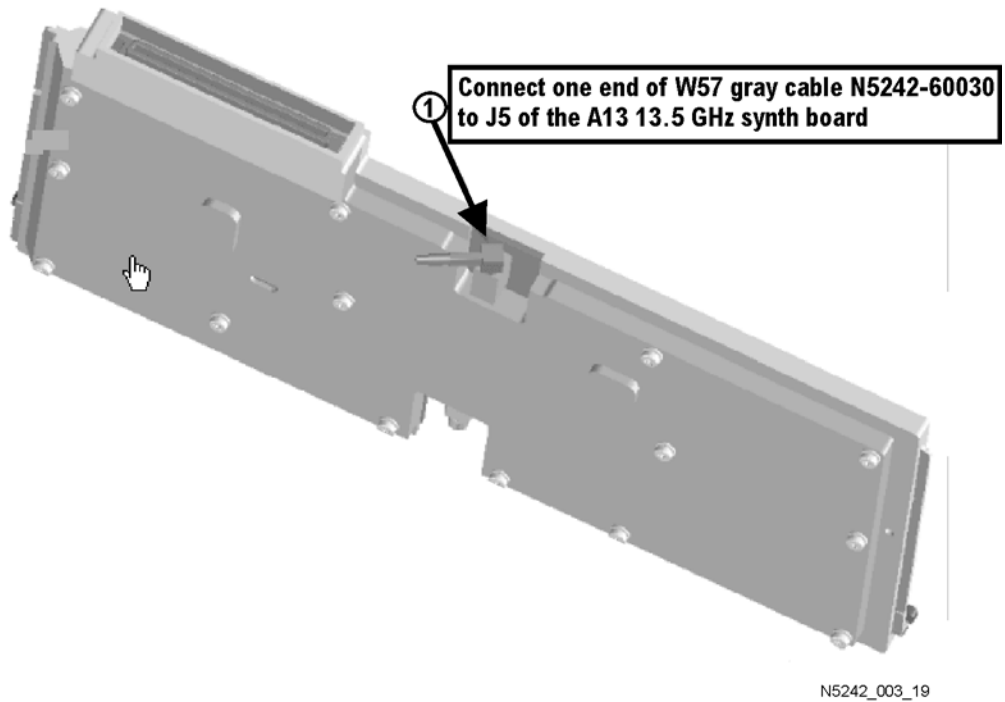
Cable Connections to the Second Source Boards, Part 1a
